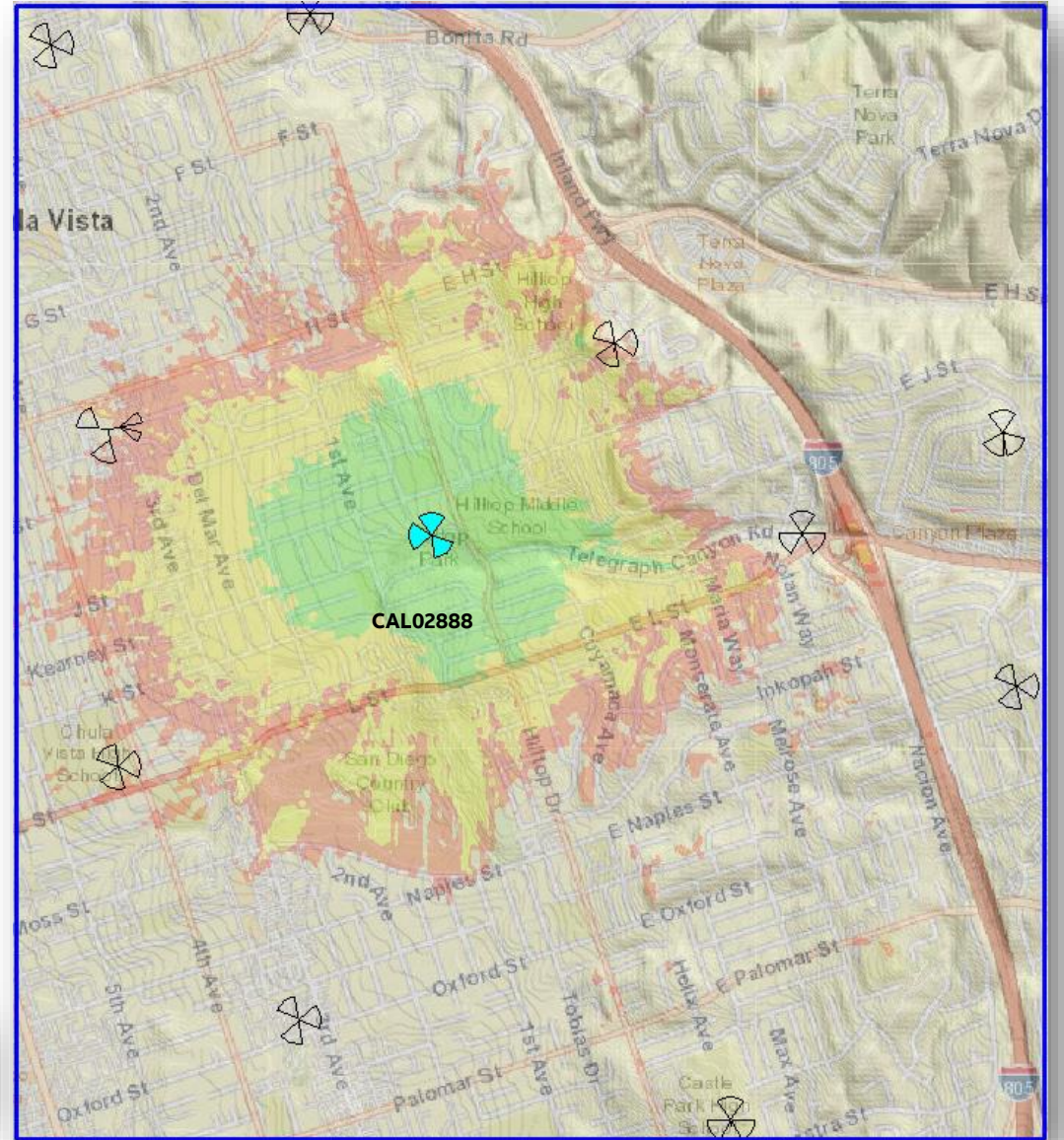
Single Site Coverage at 30 ft
