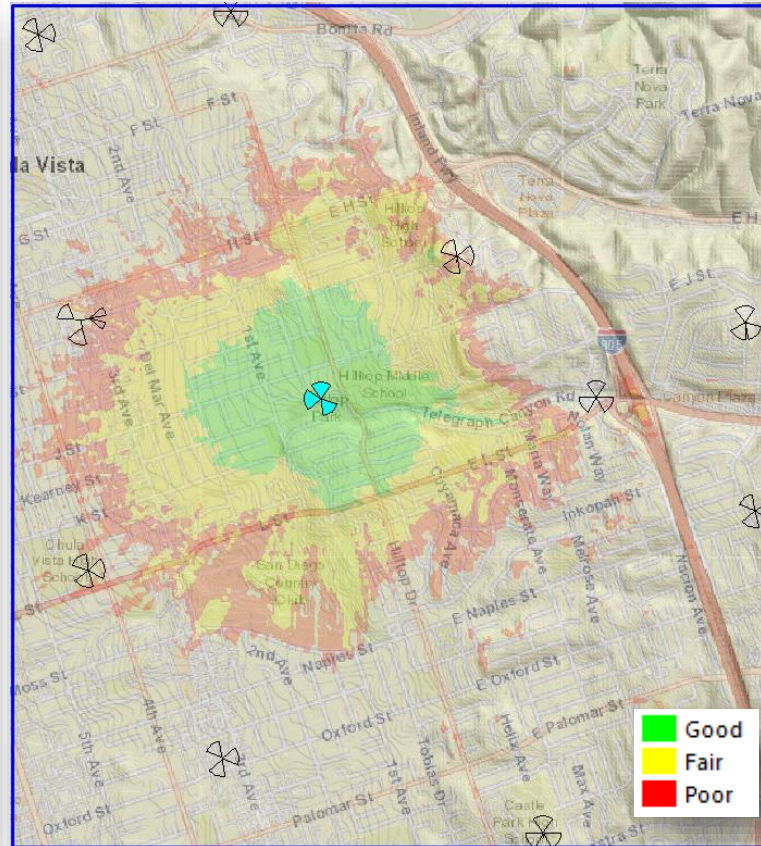
Single Site Coverage at 30 ft
