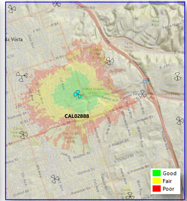
Single Site Coverage at 23 ft
