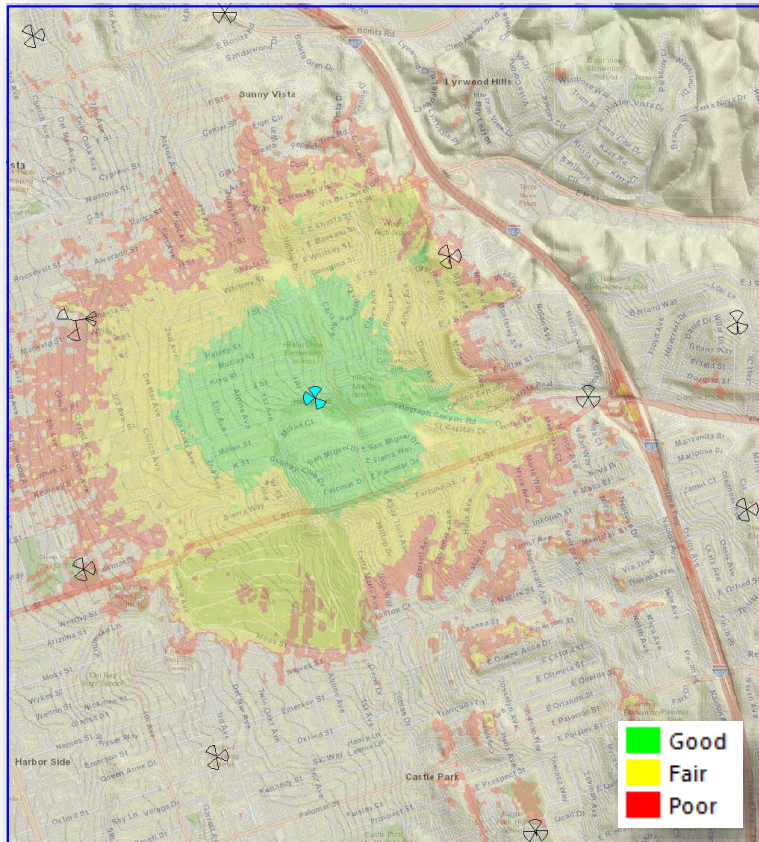
Single Site Coverage at 46 ft
