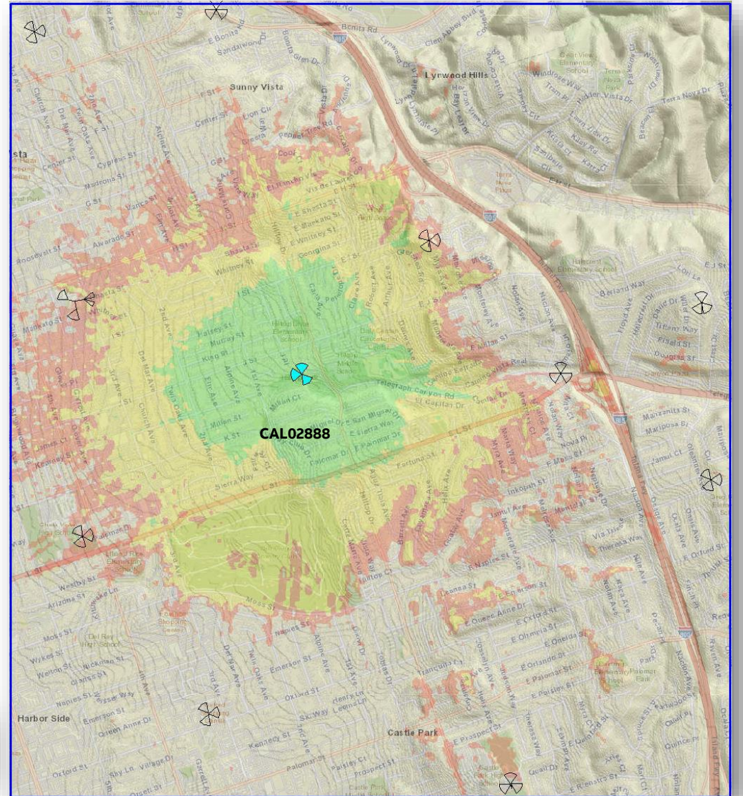
Single Site Coverage at 46 ft
