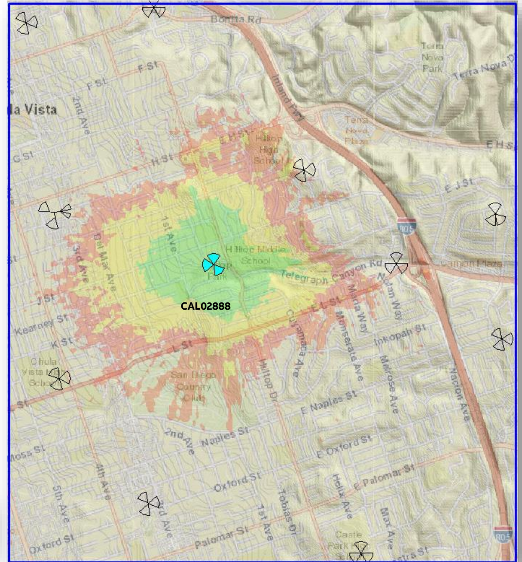
Single Site Coverage at 23 ft
